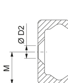
Rail with countersunk holes
