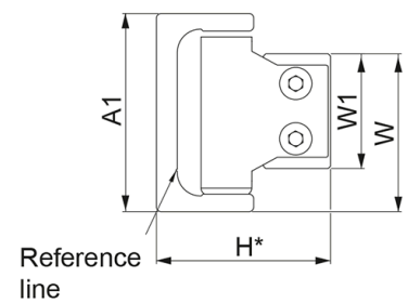
U-rail with CSW slider
