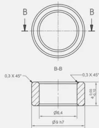
CENTERING RING CR9 Material: 1.4305 ( AISI303)
