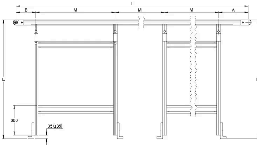
Stand TB40 Multi Timing Belt Conveyor 900 < E,D ≤ 1200
