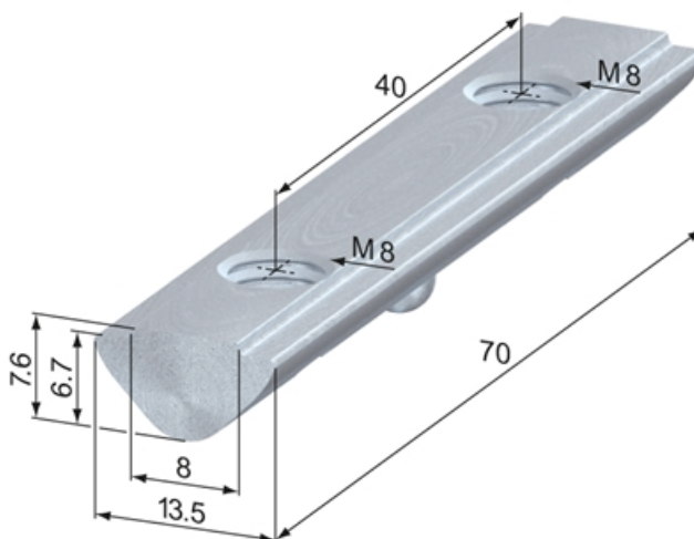
T-Nuts, slide-in
