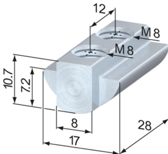
T-Nuts, slide-in
